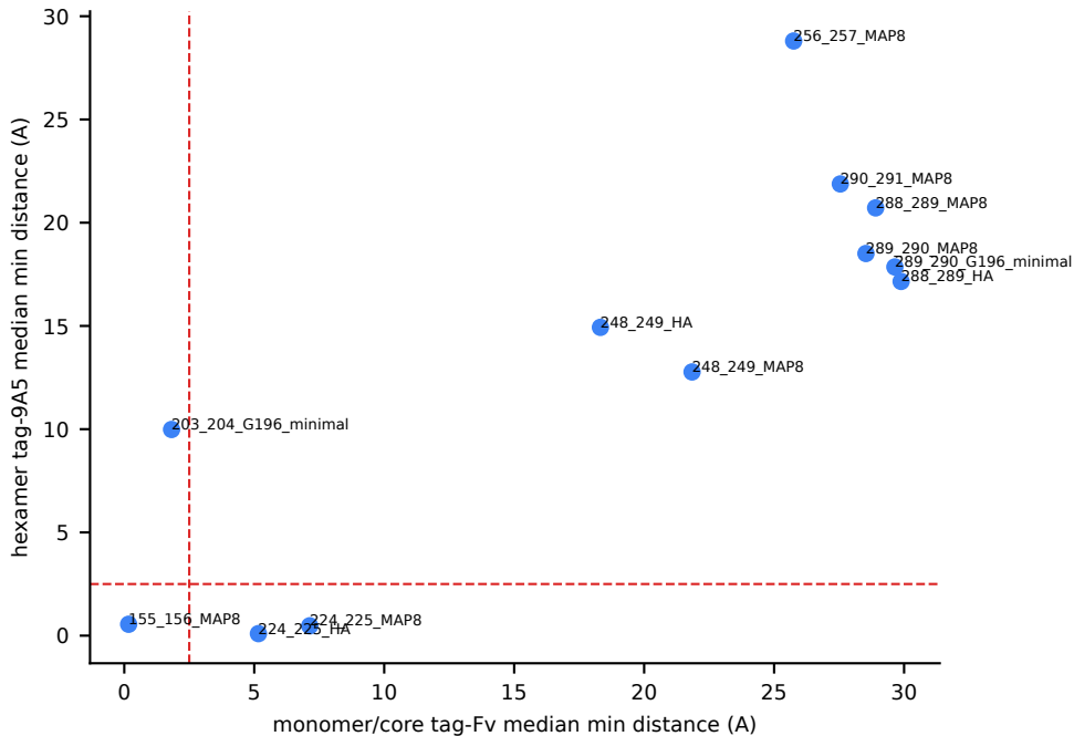
Monomer and hexamer antibody-context distances
