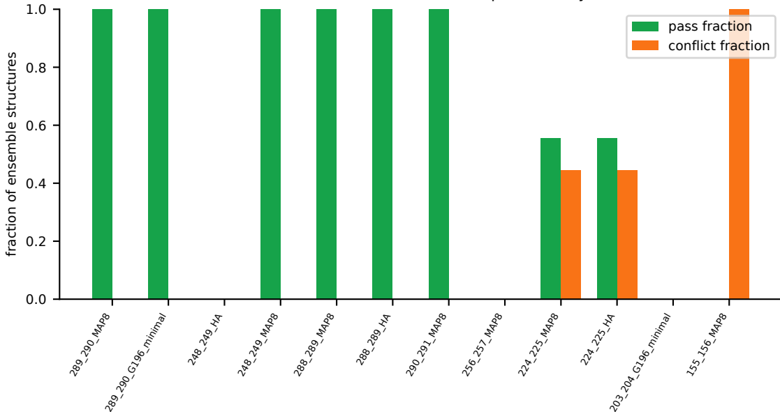
Hexamer-context ensemble reproducibility
