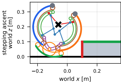
stance \theta = 60.0^\circ, \beta = -20^\circ
