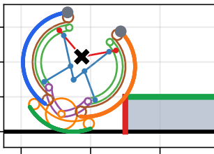
front-face contact \theta = 60.0^\circ, \beta = -20^\circ
