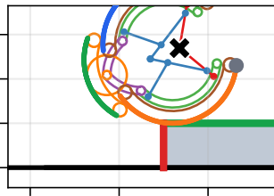
top contact \theta = 60.0^\circ, \beta = -70^\circ
