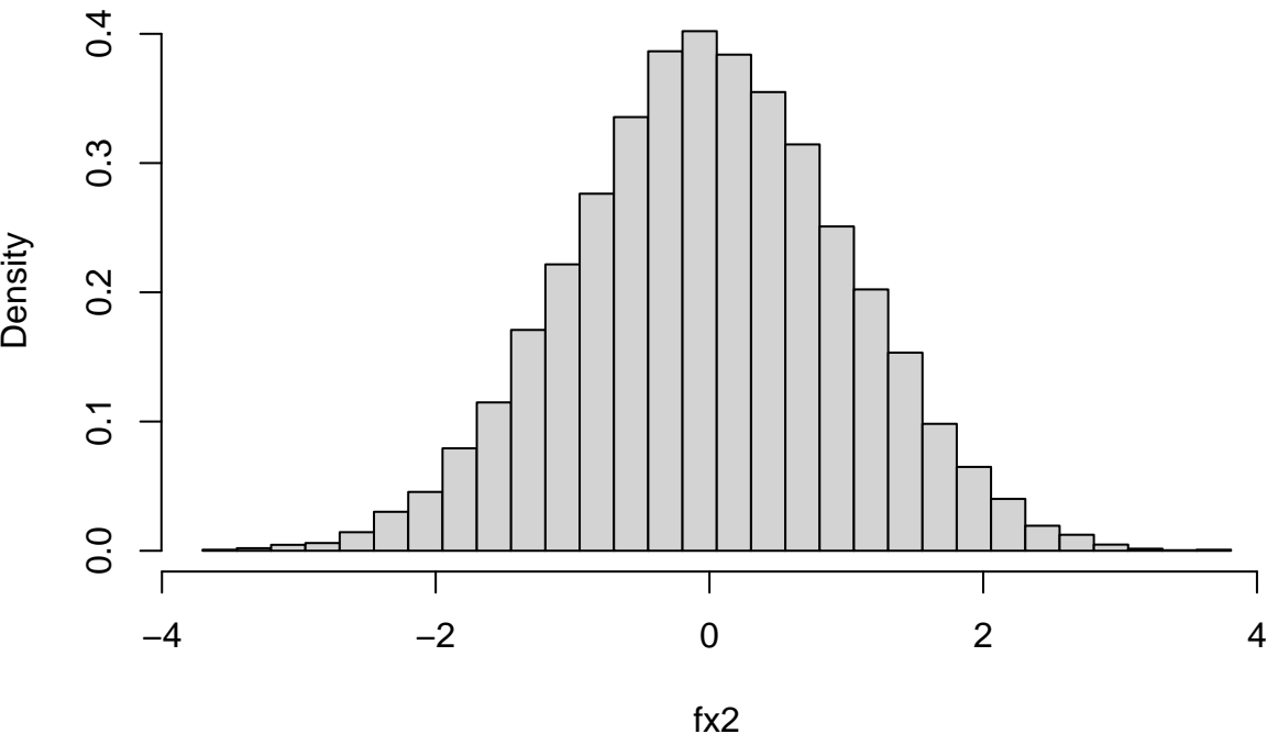
Histogram of fx2
