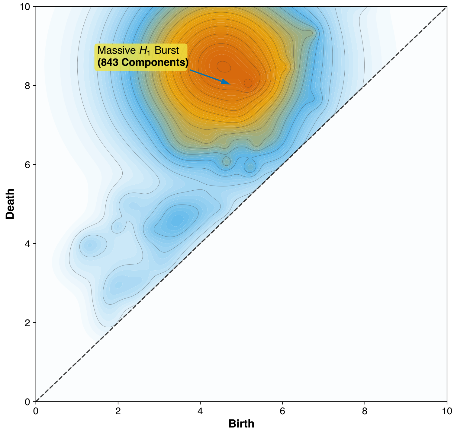
Topological Persistence of Hepatitis B Reticulation ( \beta_1 = 843 )
