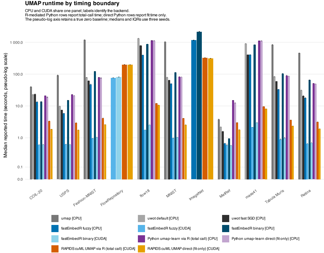
Figure 2: Runtime for the available UMAP implementations. The single panel combines CPU and CUDA results, identified in the legend, for the R umap package, uwot default and fast-SGD modes, fastEmbedR fuzzy and binary modes, Python umap-learn, and RAPIDS cuML UMAP. Colors follow Figure 1; R-mediated Python rows again report total elapsed R-call time, and direct-Python rows report Python fit time only. These timing scopes are labeled separately and are not pooled. The pseudo-log runtime axis likewise retains a true zero baseline. Binary fastEmbedR results are an explicitly labeled adjacency-only approximation; fuzzy mode is the standard comparison. Unmatched FlowRepository and ImageNet rows are descriptive only.
