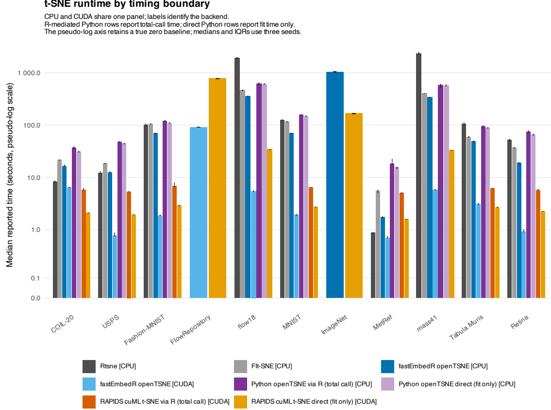
Figure 1: Runtime for the available t-SNE implementations. The single panel includes CPU and CUDA results, identified explicitly in the legend, for Rtsne , FIt-SNE , fastEmbedR openTSNE , Python openTSNE , and RAPIDS cuML t-SNE . Gray denotes established R references, blue denotes fastEmbedR , purple denotes Python openTSNE , and orange denotes RAPIDS ; shades distinguish backend or timing interface. The continuous pseudo-log runtime axis retains a true zero baseline. Bars are medians over seeds 4, 17, and 42; error bars span the interquartile range. R-mediated Python rows report total elapsed R-call time, including conversion and transfer, whereas direct-Python rows report Python fit time only; the two timing boundaries remain separate in the figure and archived tables. Missing or failed rows remain in the supplementary result files. Unmatched FlowRepository and ImageNet rows are descriptive only and excluded from comparative summaries.
