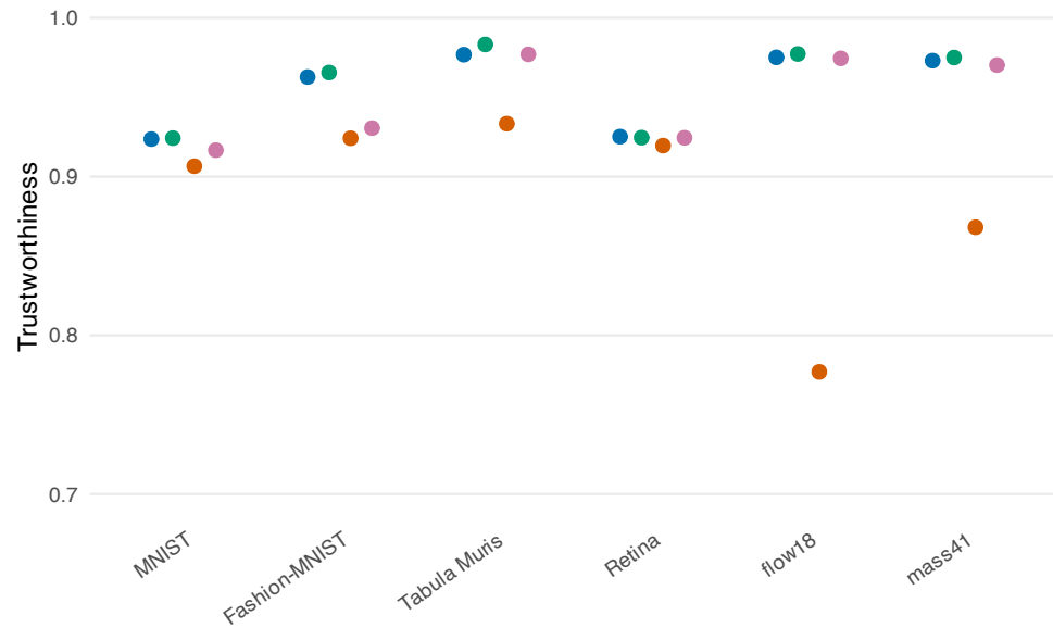
B t-SNE quality
