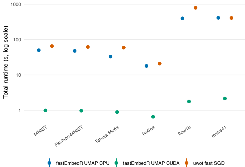
C UMAP total runtime
