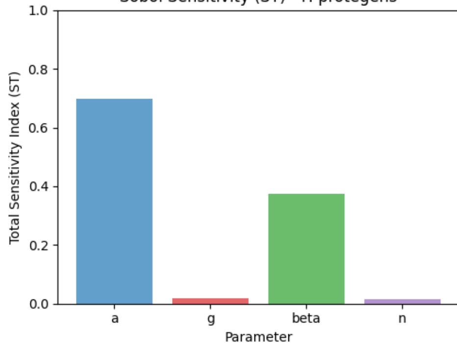
Sobol Sensitivity (ST) - P. protegens
