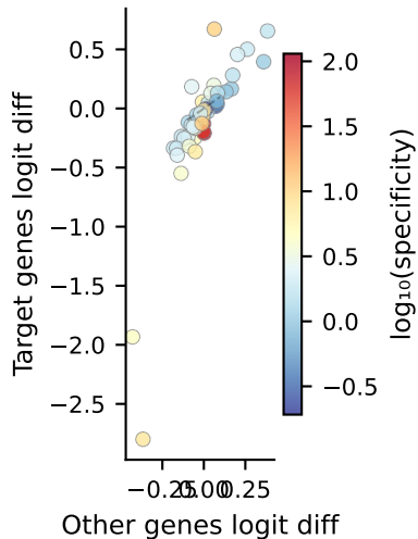
B Target vs other effect
