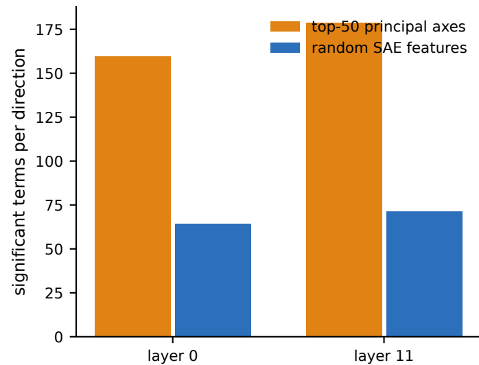
c Annotation yield per direction
