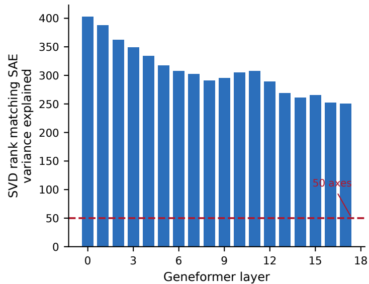
b Reconstruction-matched capacity
