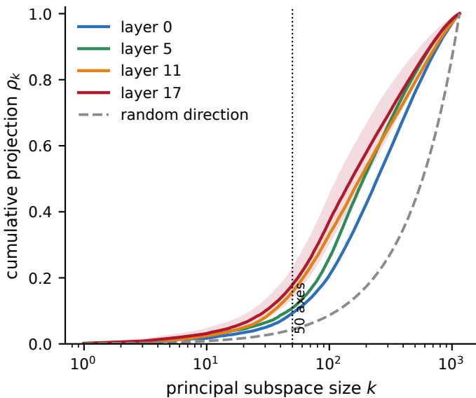
a SAE directions within the principal subspace
