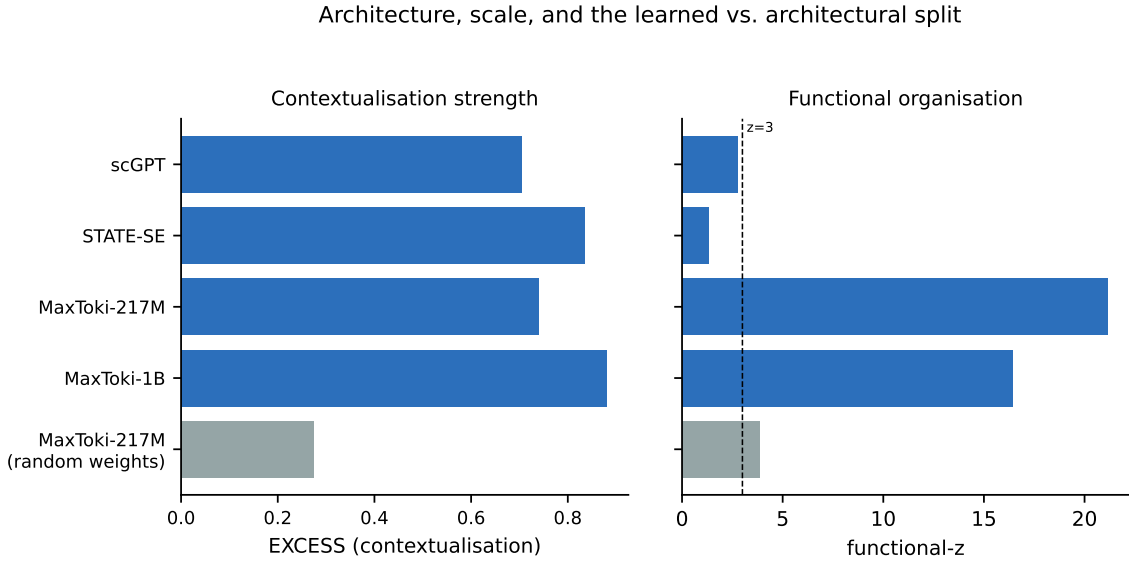
Figure 5: Figure 5. Contextualisation as a model metric across architecture, scale, and the random-weights control.
