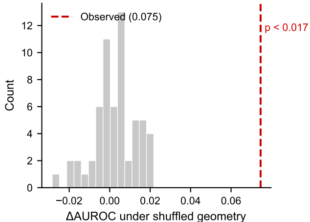
B Geometry-shuffle null (kidney, L5)
