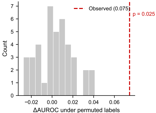
A Label permutation null (kidney, L5)
