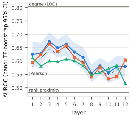
E Direction on TRRUST edges
