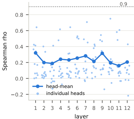
D Attention vs rank distance, co-expr.
