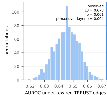
F Degree-preserving null
