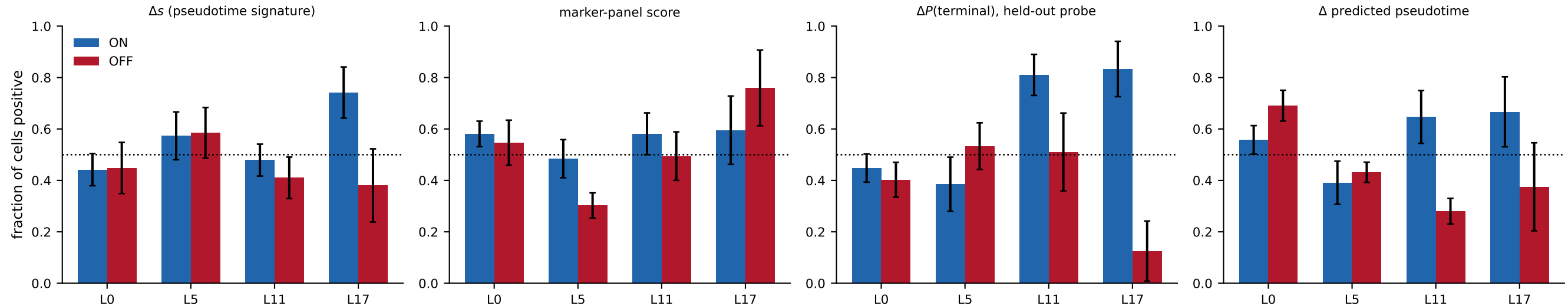
Steering directionality under four readouts ( \alpha=5 ); only the leftmost uses the pseudotime signature
