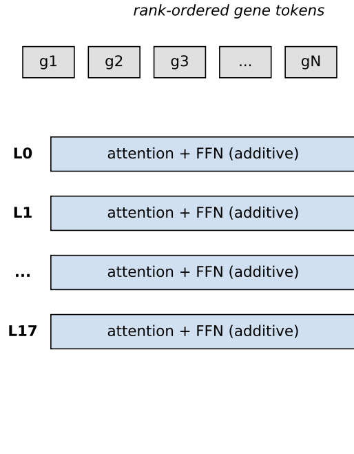
(A) Geneformer residual stream
