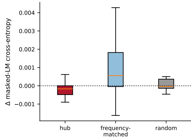
A Damage from ablating one feature
