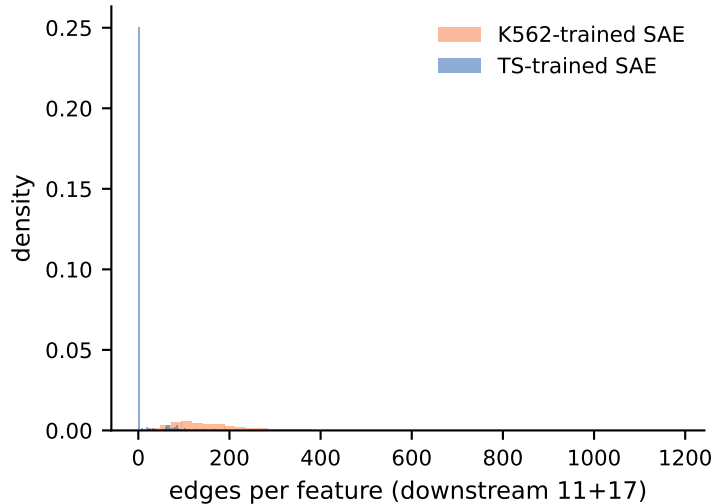
A Degree distribution
