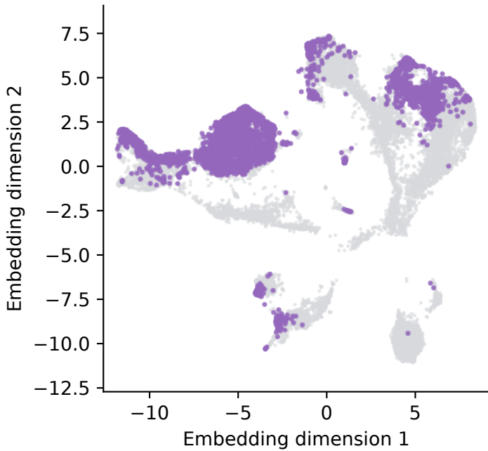
Uniform | extrapolation reference=18,486, query=6,302
