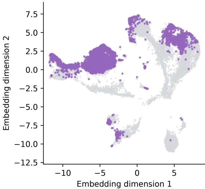
FitGrid | extrapolation reference=18,486, query=6,302
