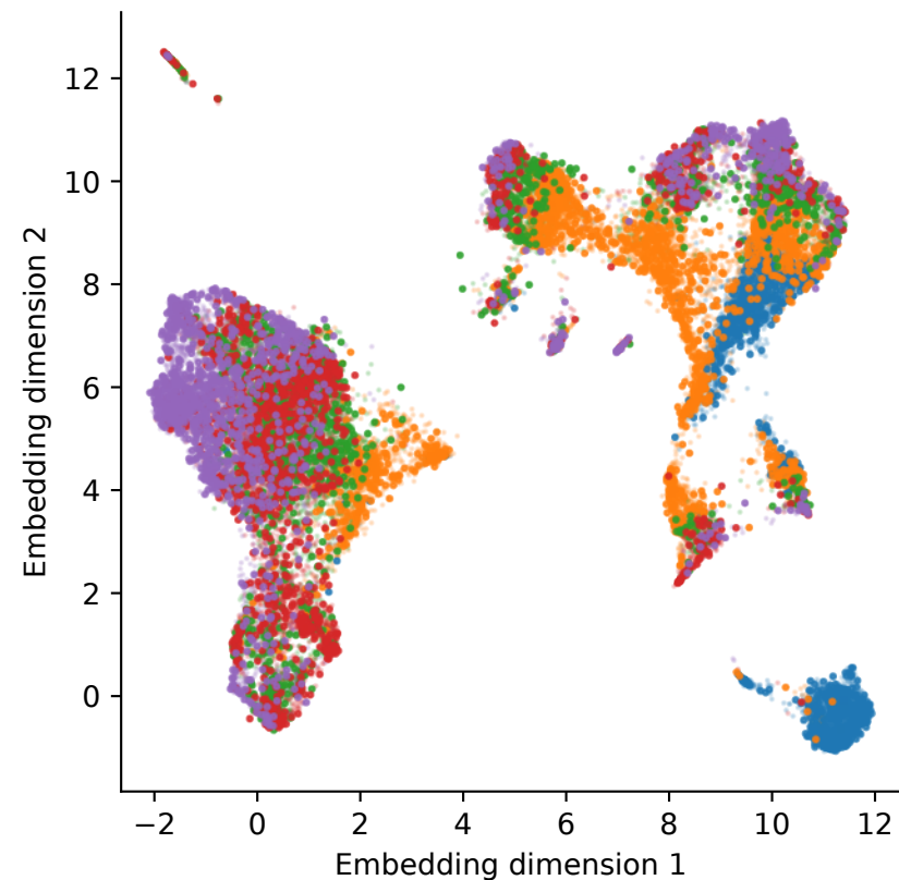
Standard UMAP | all reference=24,823, query=6,206
