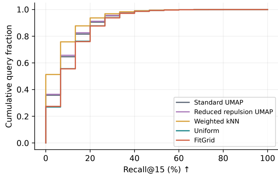
all | n=12543
