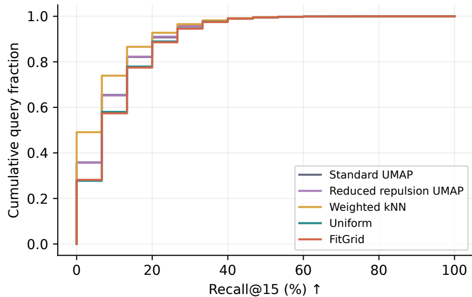
interpolation | n=6241
