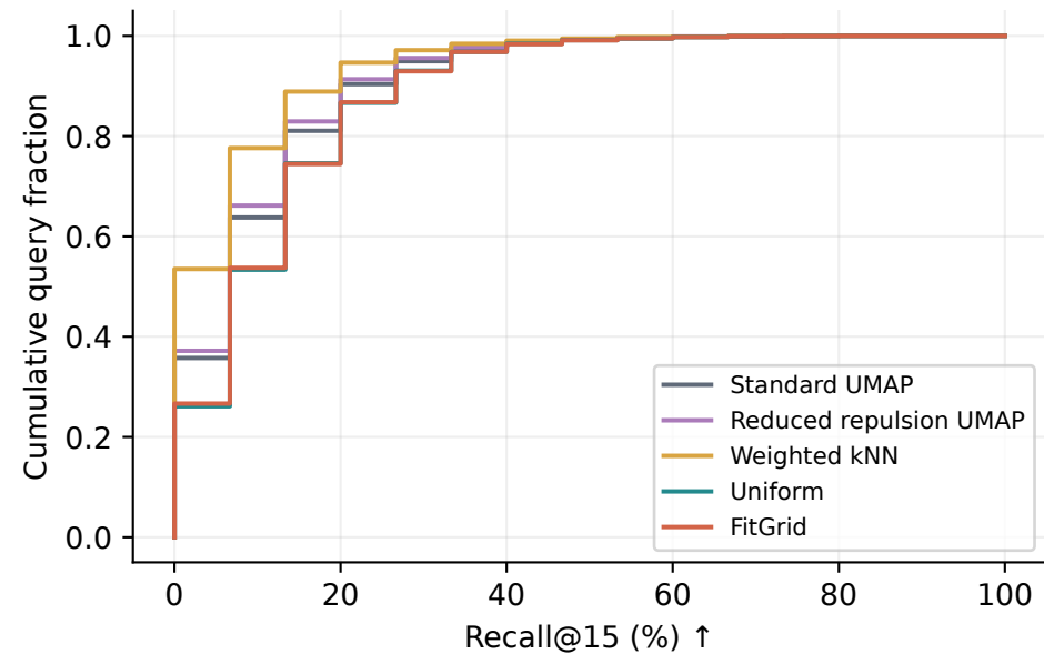
extrapolation | n=6302
