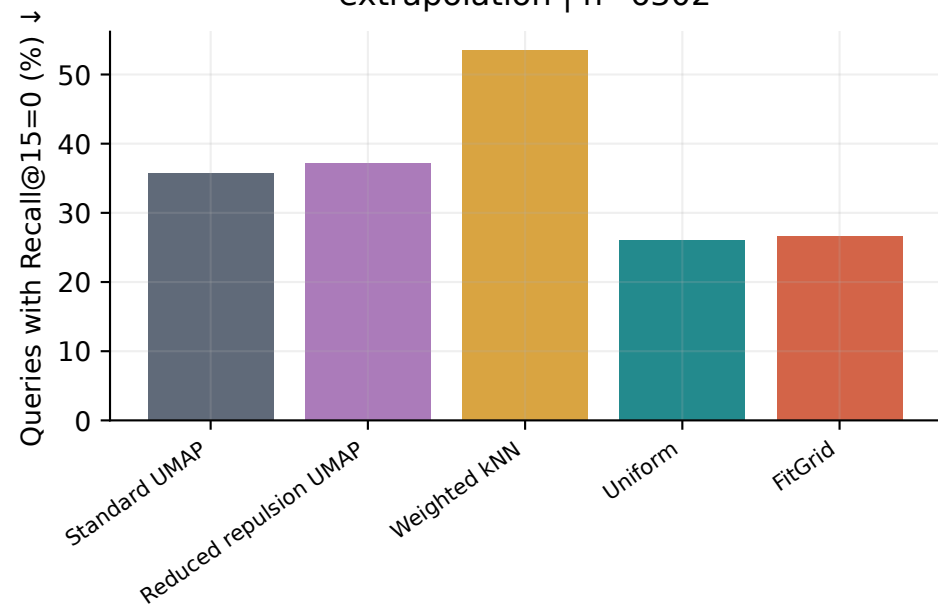
extrapolation | n=6302
