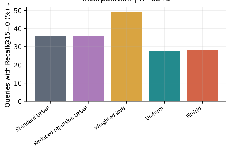
interpolation | n=6241
