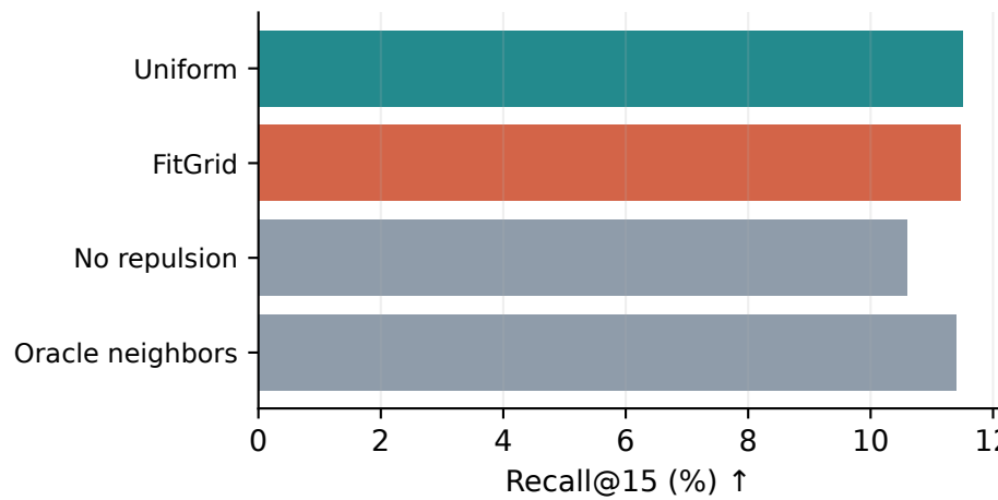
extrapolation | n=6302
