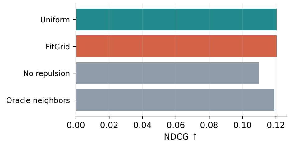
extrapolation | n=6302
