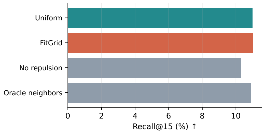
interpolation | n=6241
