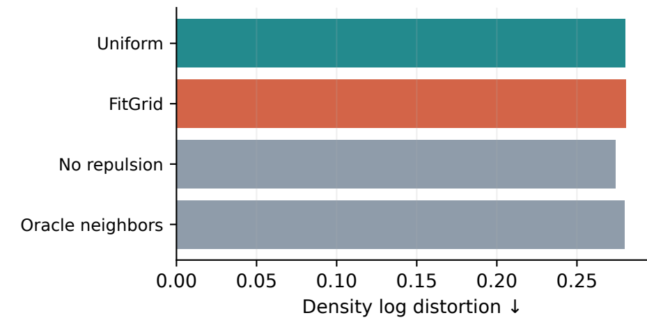
interpolation | n=6241
