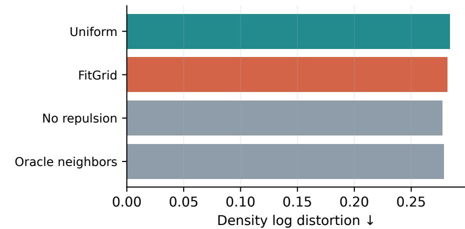
extrapolation | n=6302
