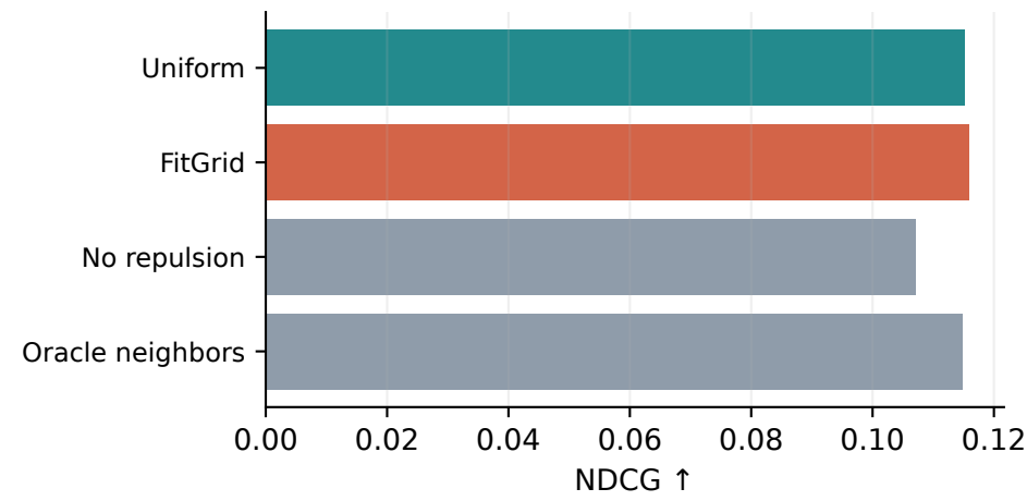
interpolation | n=6241
