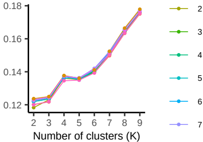
Silhouette score
