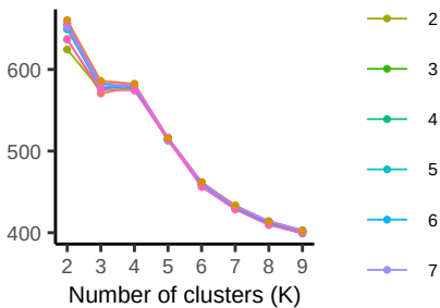
Calinski-Harabasz index
