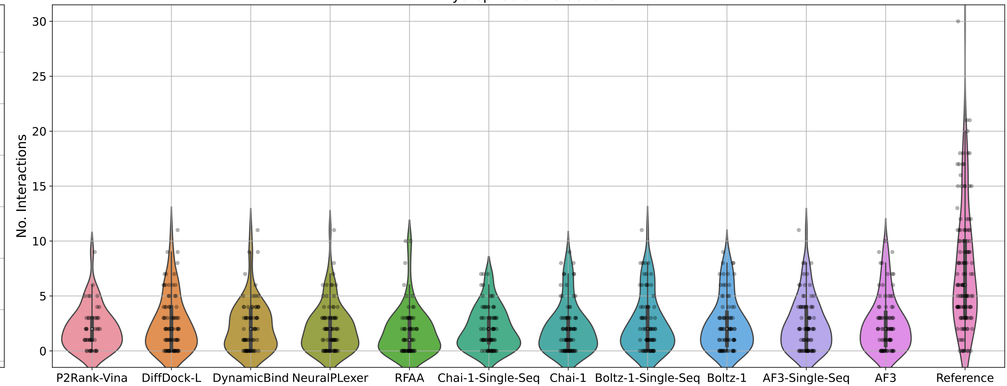
Hydrophobic Interactions
