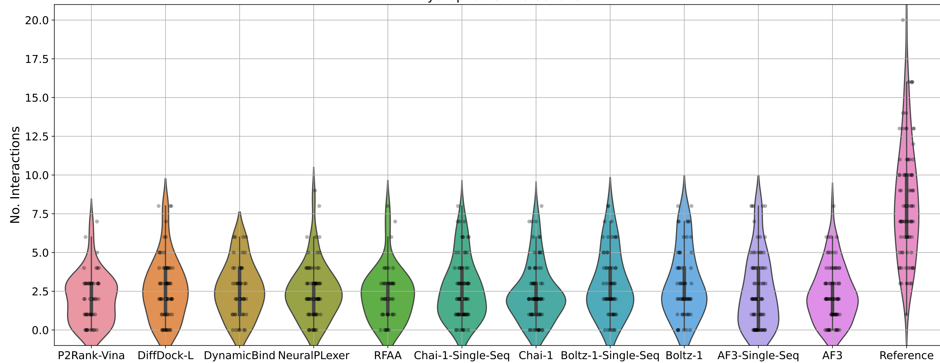
Hydrophobic Interactions
