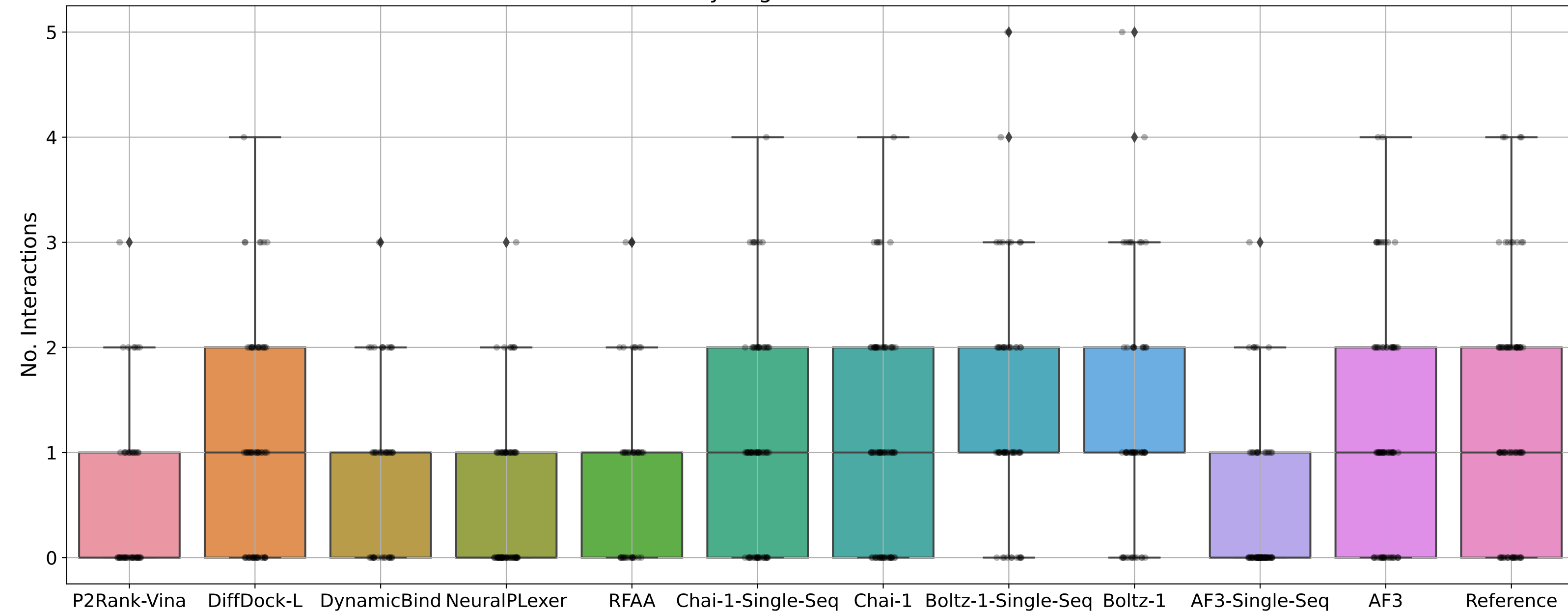
Hydrophobic Interactions
