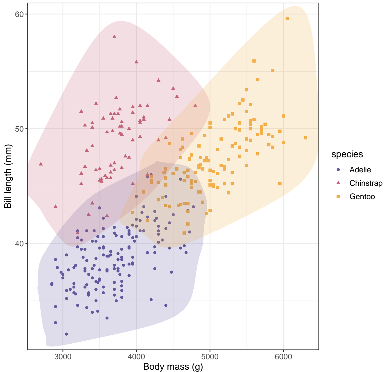
Palmer penguin body mass and bill length distribution by species
