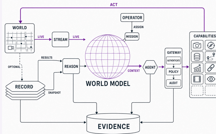
Figure 1. The harness loop. Stream processes live media directly, recording is optional, and every agent action passes the gateway's authentication, policy, and audit checks.
