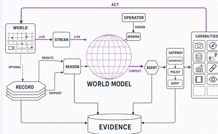
Figure 1. The harness loop. Stream processes live media directly, recording is optional, and every agent action passes the gateway's authentication, policy, and audit checks.
