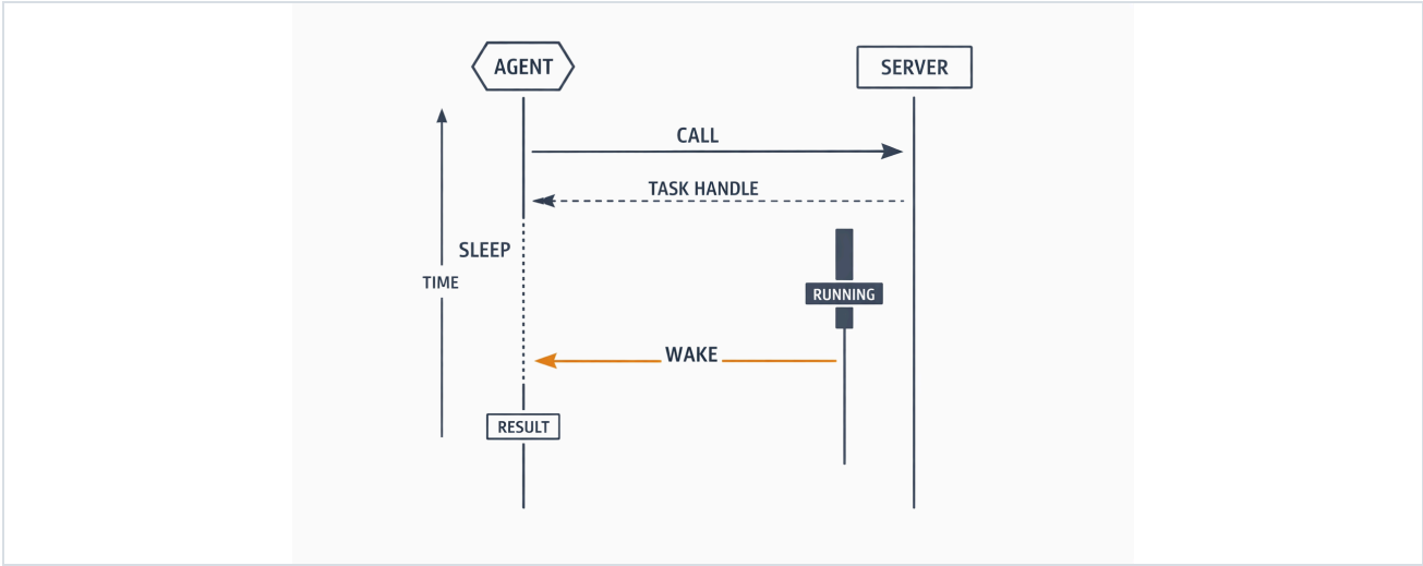
FIGURE 8 – DETACH → SLEEP → WAKE: ZERO CONNECTIONS HELD, ZERO EPISODES BURNED WAITING.
