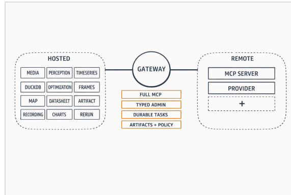
FIGURE 5 – TWELVE HOSTED SERVERS AND REMOTE ENDPOINTS; FULL MCP, TYPED ADMINISTRATION, DURABLE TASKS, ARTIFACTS, AND POLICY REMAIN ONE GOVERNED SYSTEM.
