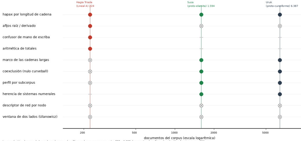
Fig. 1. At what corpus size each instrument begins to see. Filled circle: it detects the structure; cross: it does not, or the fixed-margin null reproduces it; dash: not applicable. Co-exclusion, the frame of long strings and the profile by subcorpus appear between 800 and 1,600 documents; affixes and arithmetic already work at 224; the hand control only where scribes are attributed.
