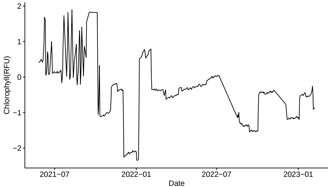
Post-QC B2O Chlorophyll(RFU) Mean Daily Value from 2021-2023
