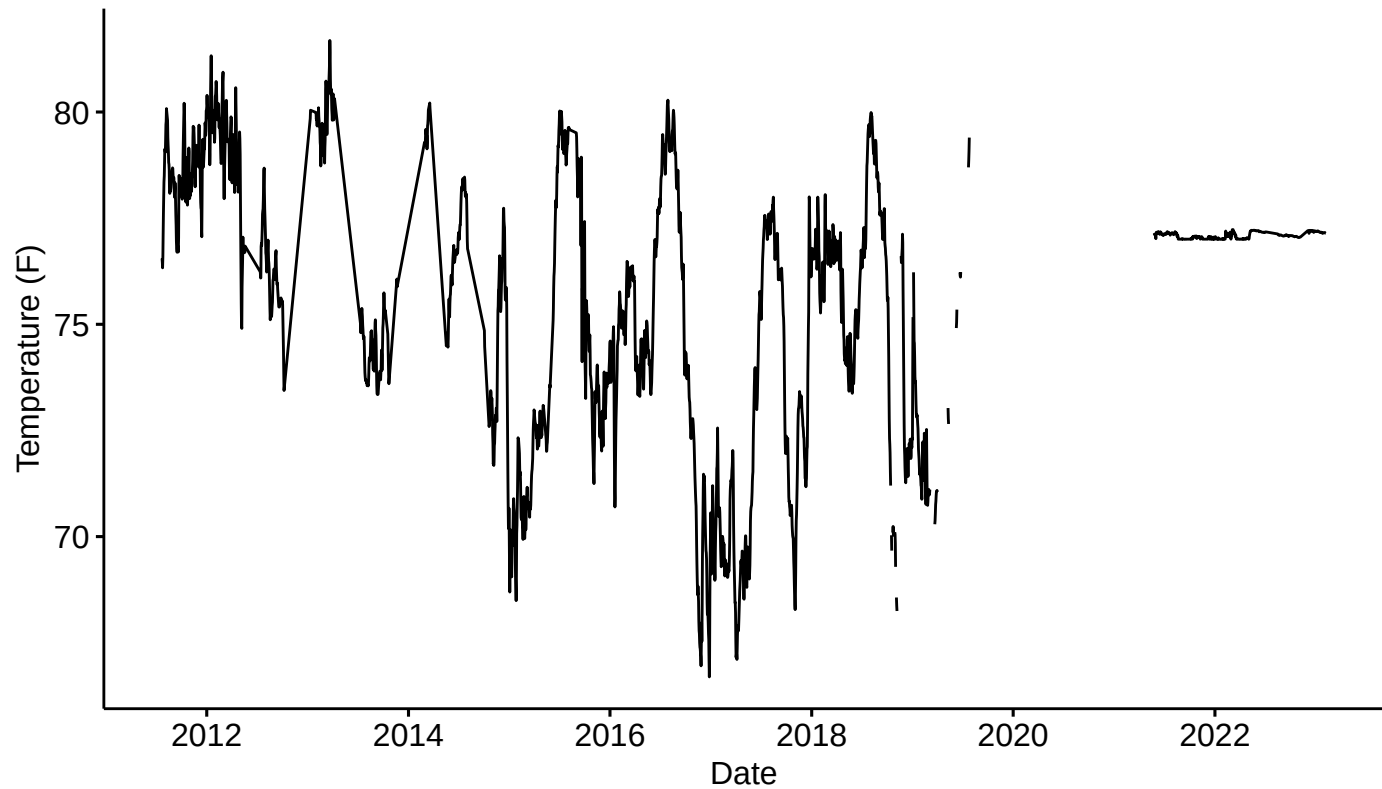
Post-QC B2O Temperature(F) Mean Daily Value from 2011-2023
