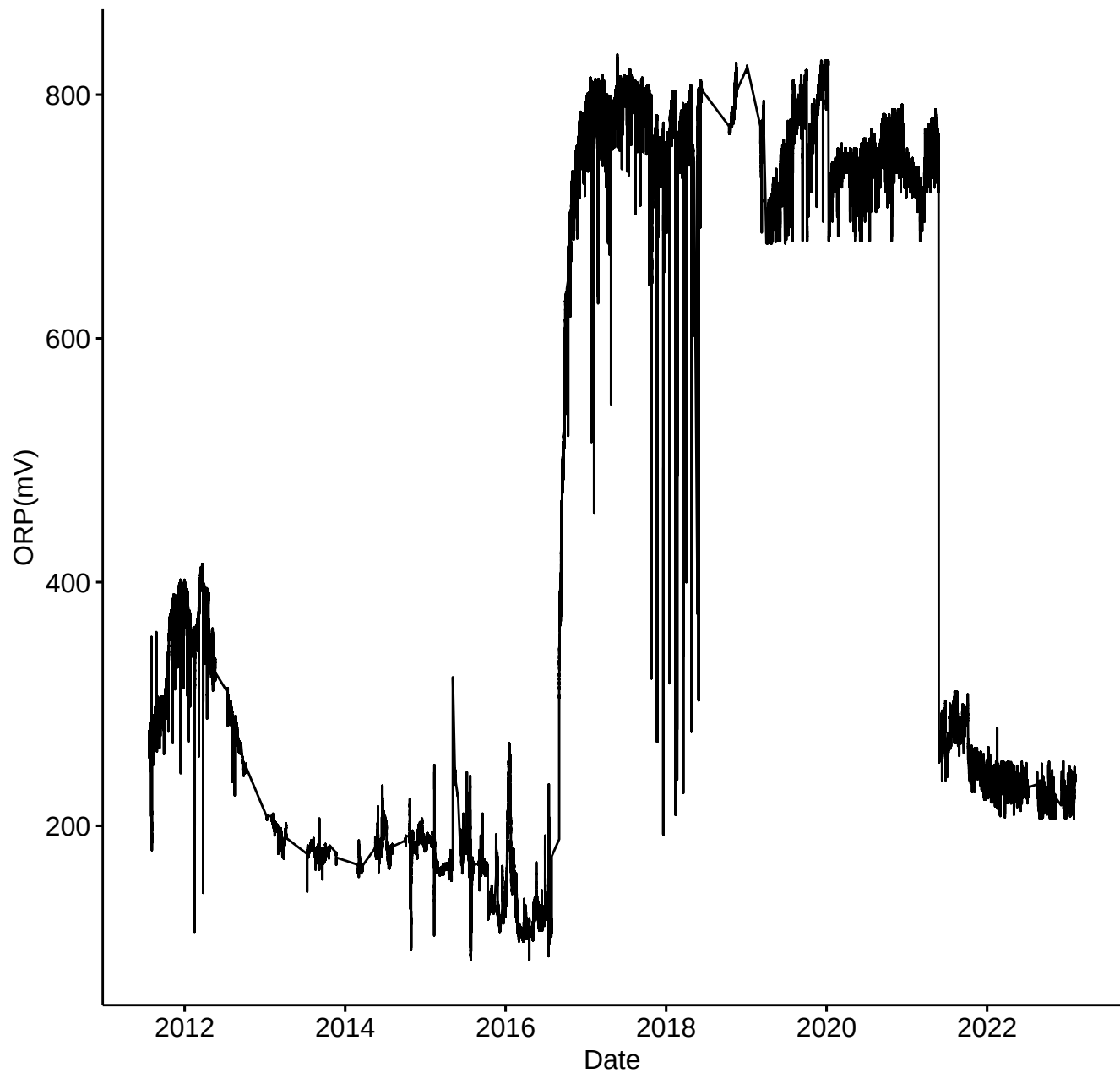
Post-QC B2O Oxidation-Reduction Potential(mV) from 2011-2023
