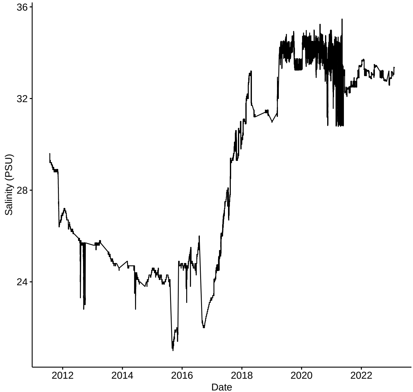
PostQC B2O Salinity(PSU) from 2011–2023
