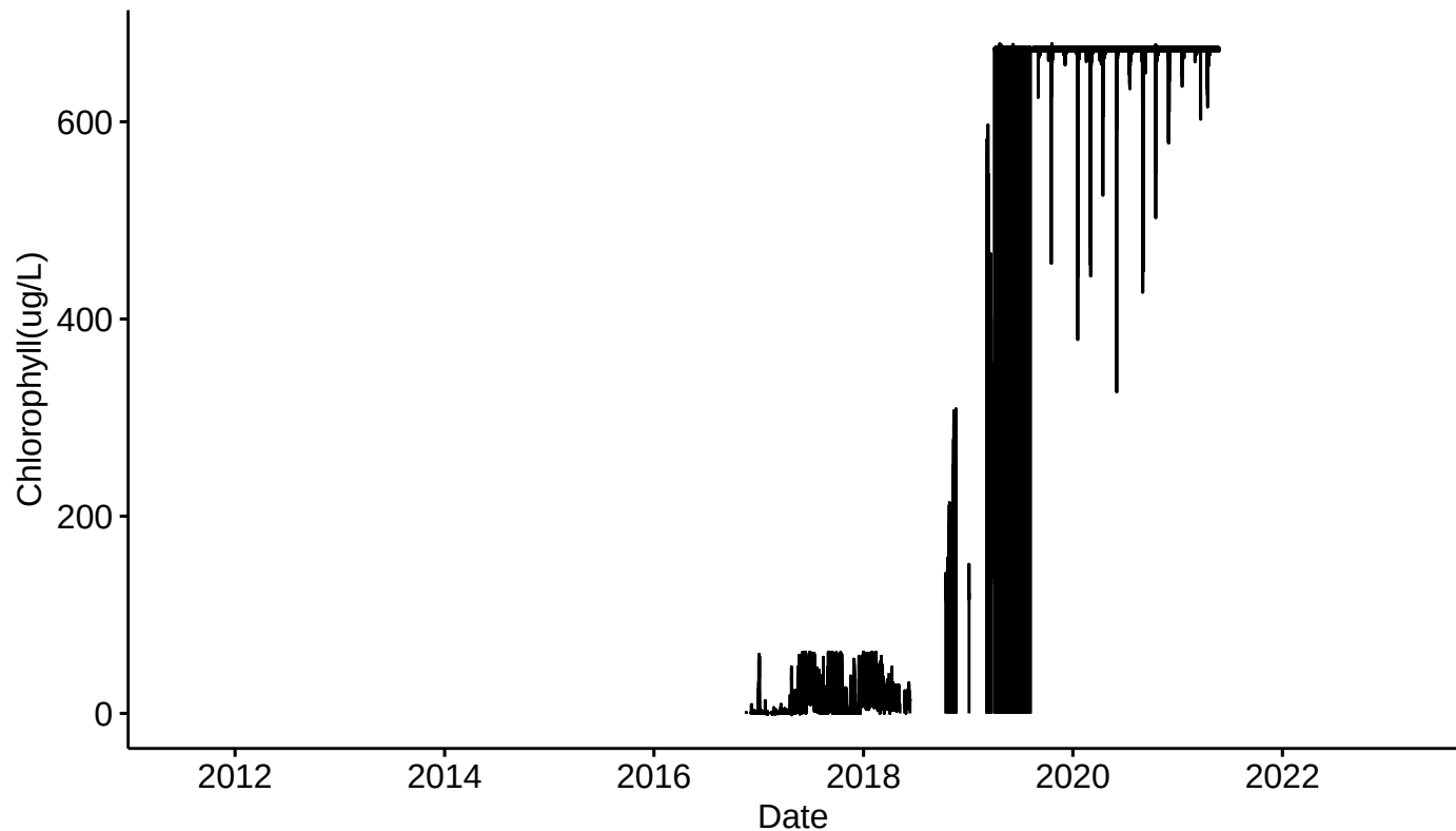
Pre-QC B2O Chlorophyll(ug/L) from 2011–2023
