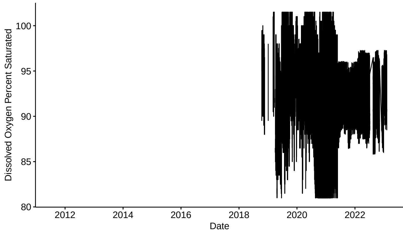
Pre-QC B2O Dissolved Oxygen Percent Saturated from 2011–2023
