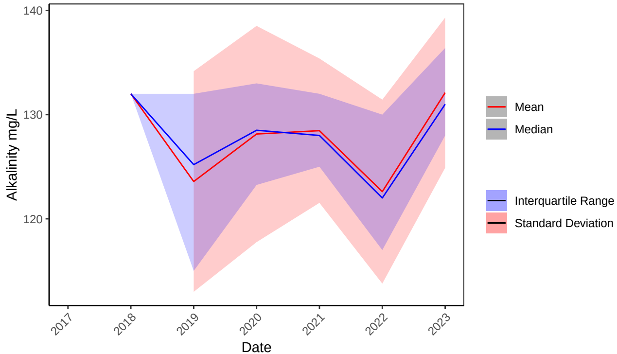
B2 Ocean Alkalinity mg/L Yearly Statistics
