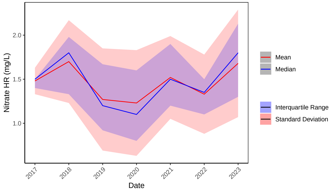
B2 Ocean Nitrate HR (mg/L) Yearly Statistics
