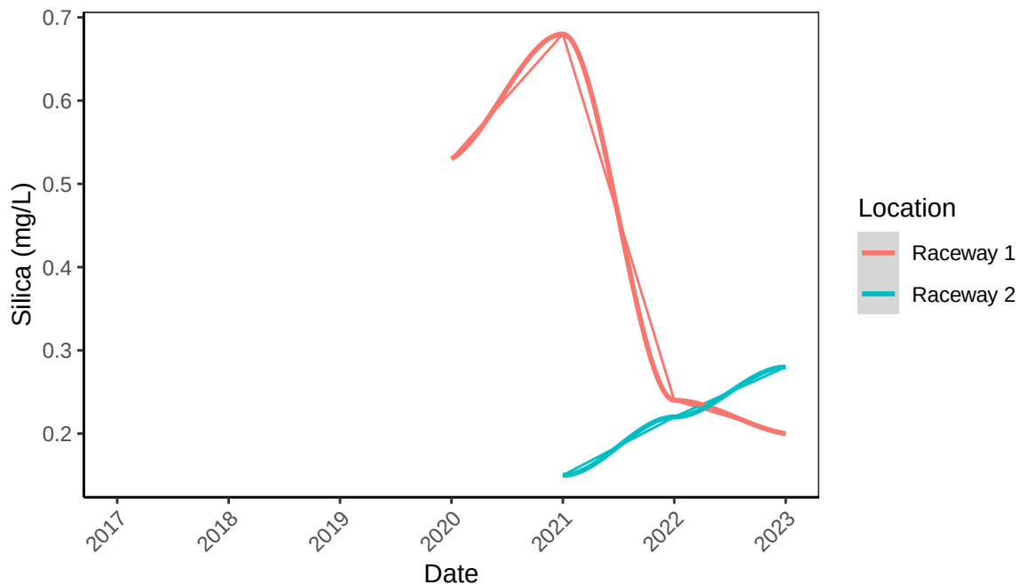
B2 Coral Raceways 1 and 2 Silica (mg/L) Yearly Mean
