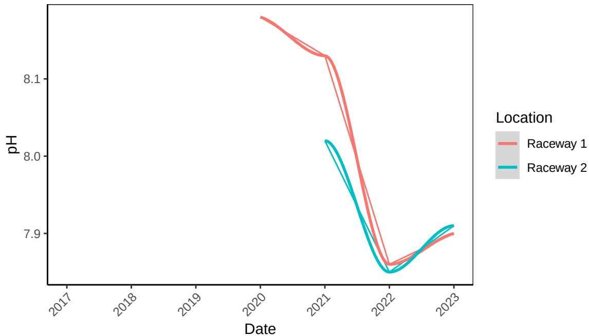
B2 Coral Raceways 1 and 2 pH Yearly Mean
