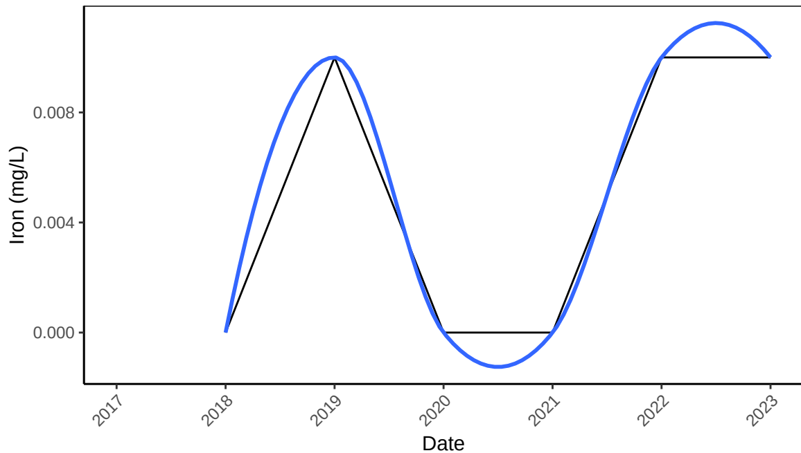
B2 Ocean Iron (mg/L) Yearly Mean
