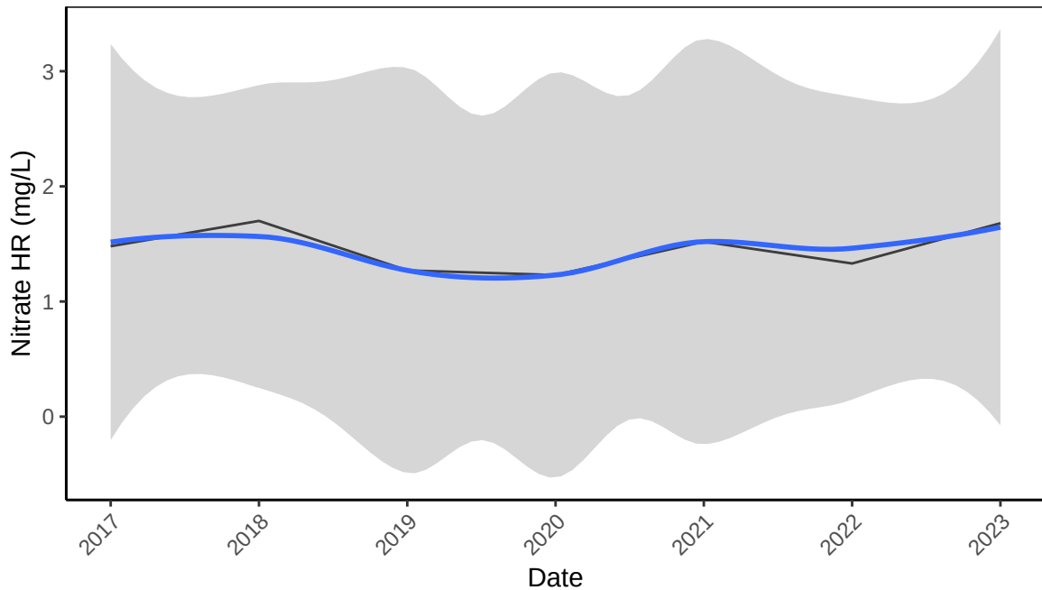
B2 Ocean Nitrate HR (mg/L) Yearly Mean
