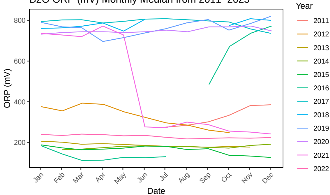
B2O ORP (mV) Monthly Median from 2011–2023
