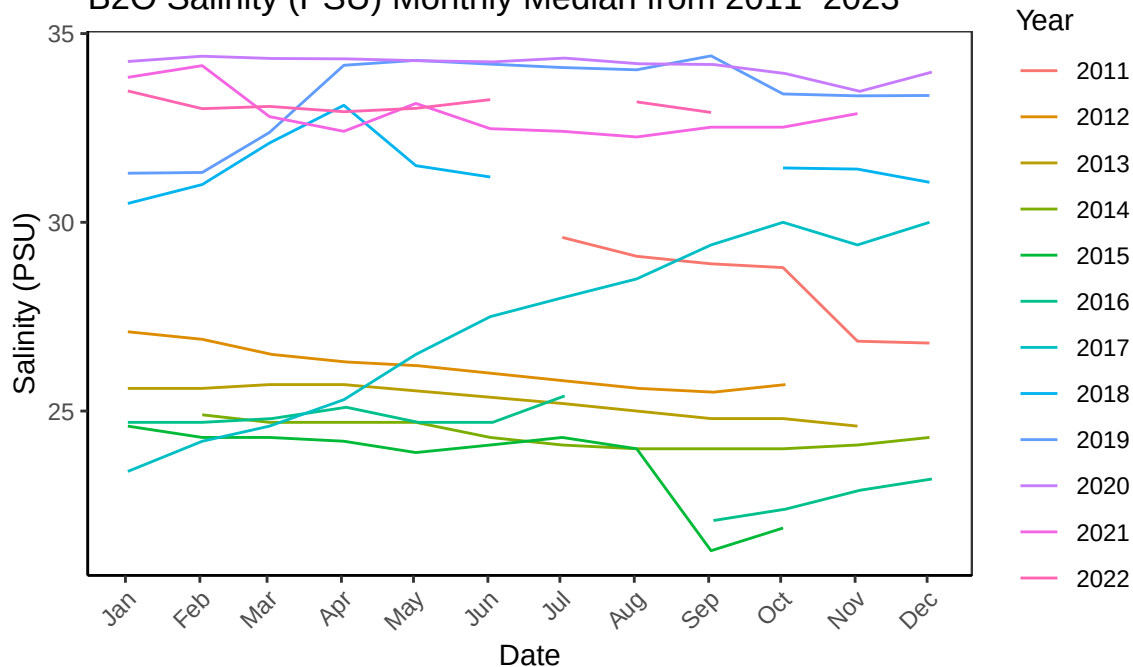
B2O Salinity (PSU) Monthly Median from 2011–2023
