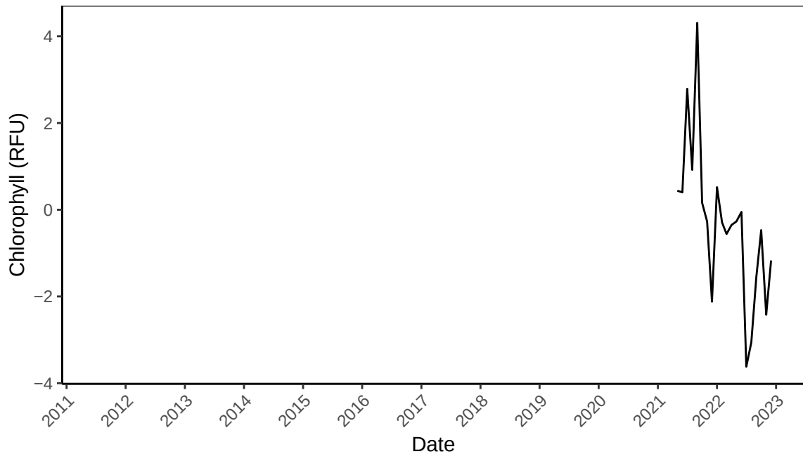
B2O Monthly Median Chlorophyll (RFU) from 2011–2023
