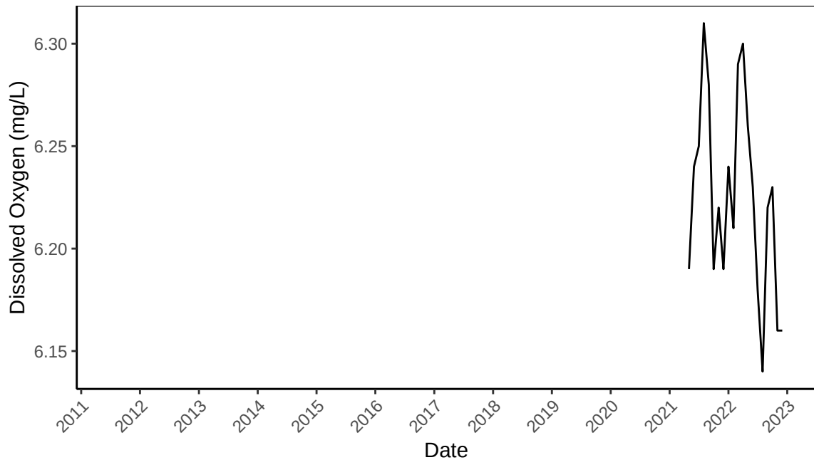
B2O Monthly Median Dissolved Oxygen (mg/L) from 2011–2023
