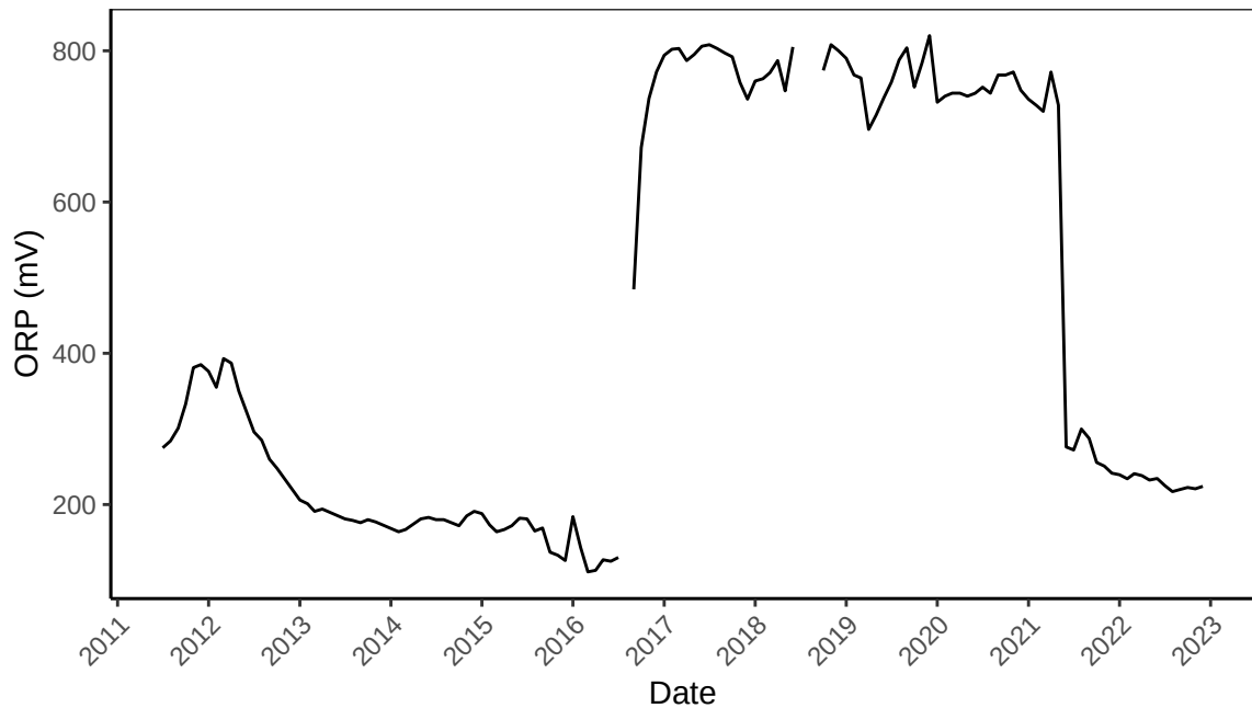
B2O Monthly Median ORP (mV) from 2011–2023
