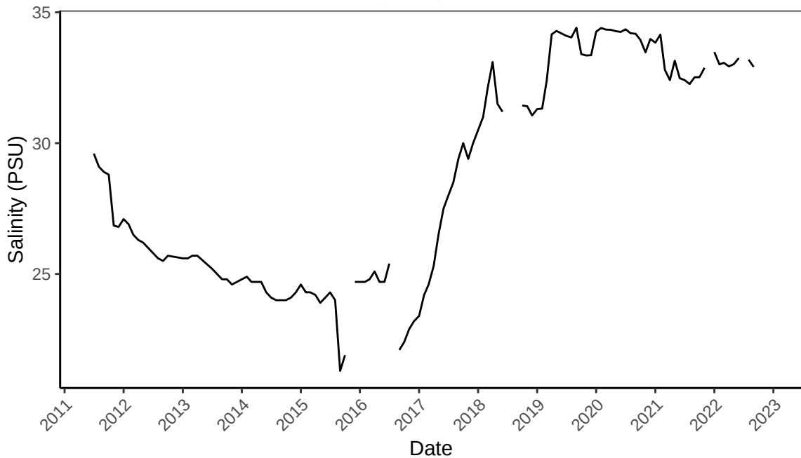
B2O Monthly Median Salinity (PSU) from 2011–2023
